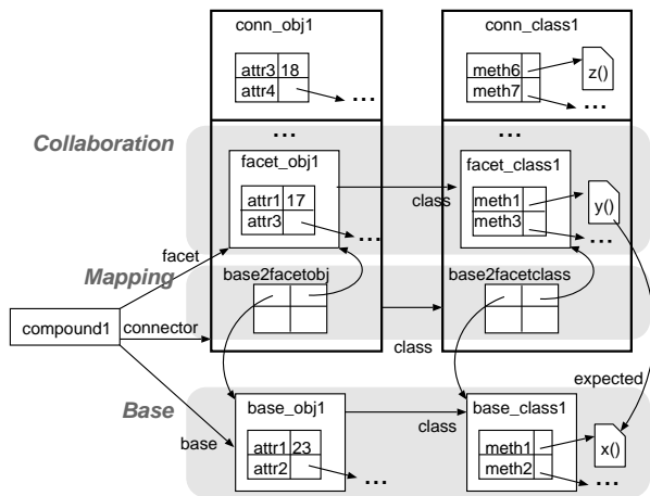
Figure 4. Run-time structures of the LAC interpreter.
